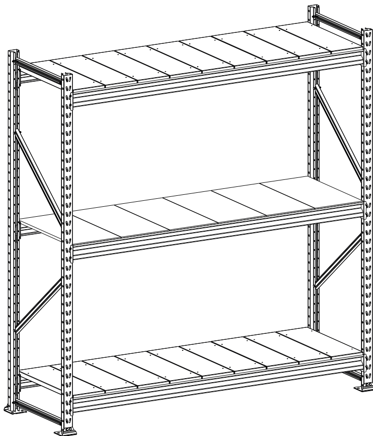
MPP 2,00m x 1,20m x 0,60m
