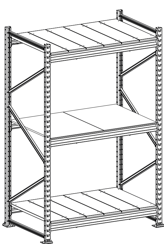
MPP 2,00m x 1,20m x 0,80m
